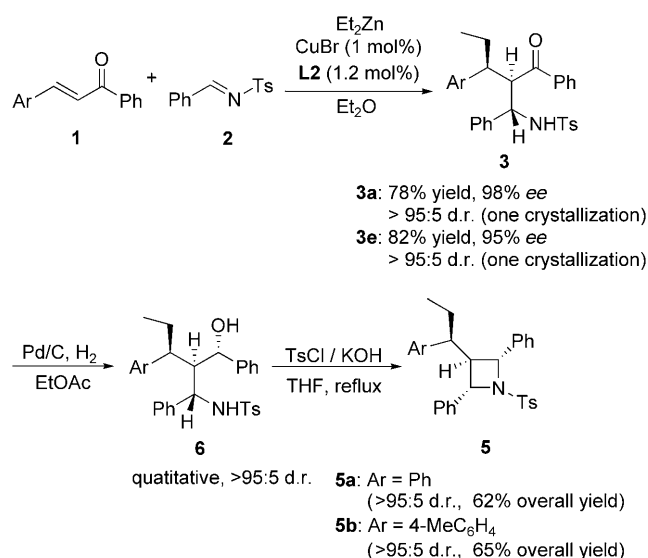
Scheme 3. Synthesis of chiral N -tosylazetidine derivatives.
