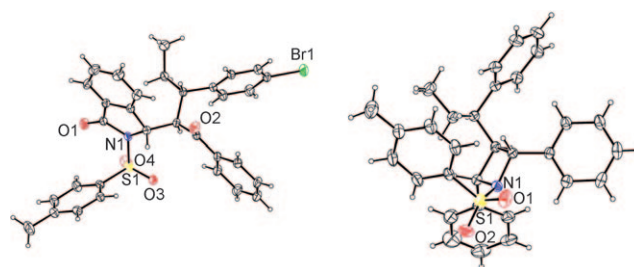
Figure 1. X-ray structures of the enantiomerically pure isoindolinone 4a (left) and azetidine 5a (right). The thermal ellipsoids are drawn at the 50 % probability level. Blue N, green Br, red O, yellow S.
