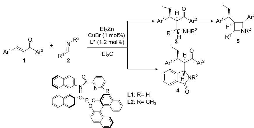
Scheme 1. Copper-catalyzed tandem conjugate addition/Mannich reaction. L* = chiral ligand.
