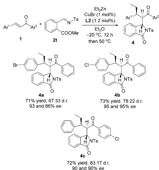
Scheme 2. Catalytic synthesis of chiral isoindolinone derivatives by a tandem reaction.
